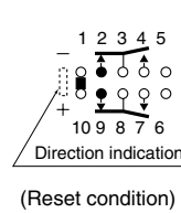
1-coil latching
